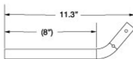
Short Flip Up Armrest
