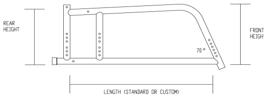
Frame Dimensions
